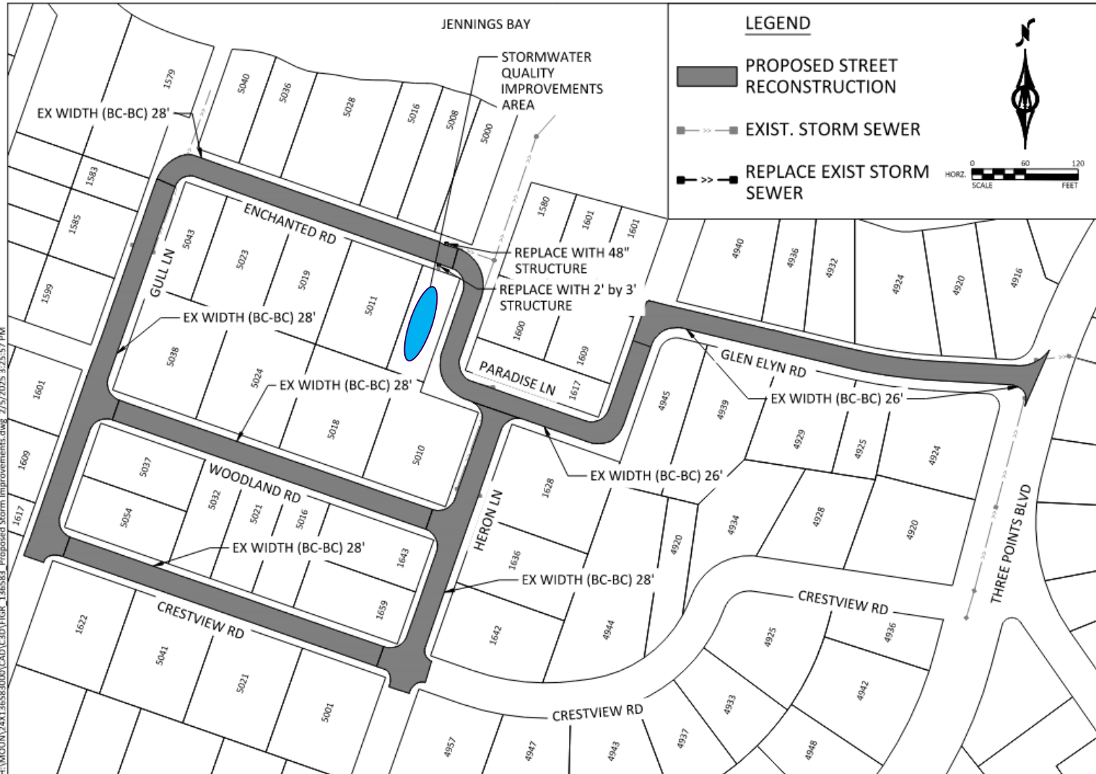
Figure 2: PROPOSED STREET IMPROVEMENTS
